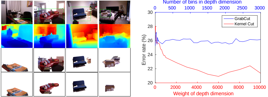
Fig. 8: NYUv2 database [42] Left: The first two rows show original images with bounding box and color-coded depth channel. The third row shows results of Grabcut, the forth row shows results of Kernel Cut. Right: The average errors of GrabCut and Kernel Cut methods over 64 images randomly selected and labeled.
