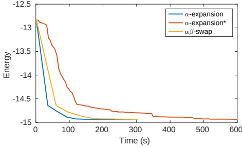
(a) Versions of Kernel Cut
