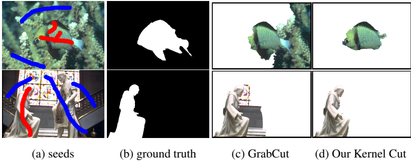
Fig. 6: Sample results on Berkeley dataset.
