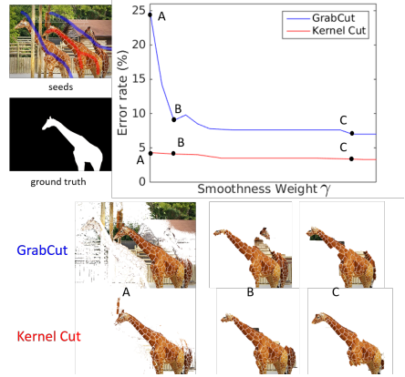
(b) Effect of smoothness weight \gamma
