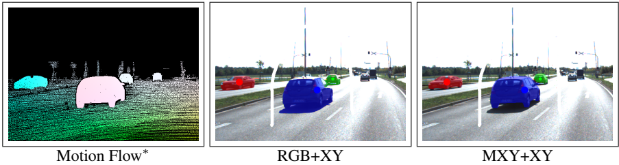
Fig. 9: Kernel cut on image 000079_10 from KITTI [43]. The images show the motion flow, color-based segmentation (RGB+XY), motion based segmentation with location features (MXY+XY). * Black color shows pixels that lack motion information.
