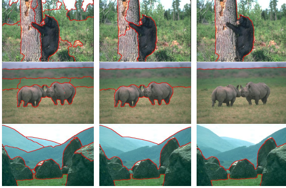
Fig. 4: Segmentation using our kernel cut with label cost. We experiment with increasing value of label cost h_k for each label (from left to right).
